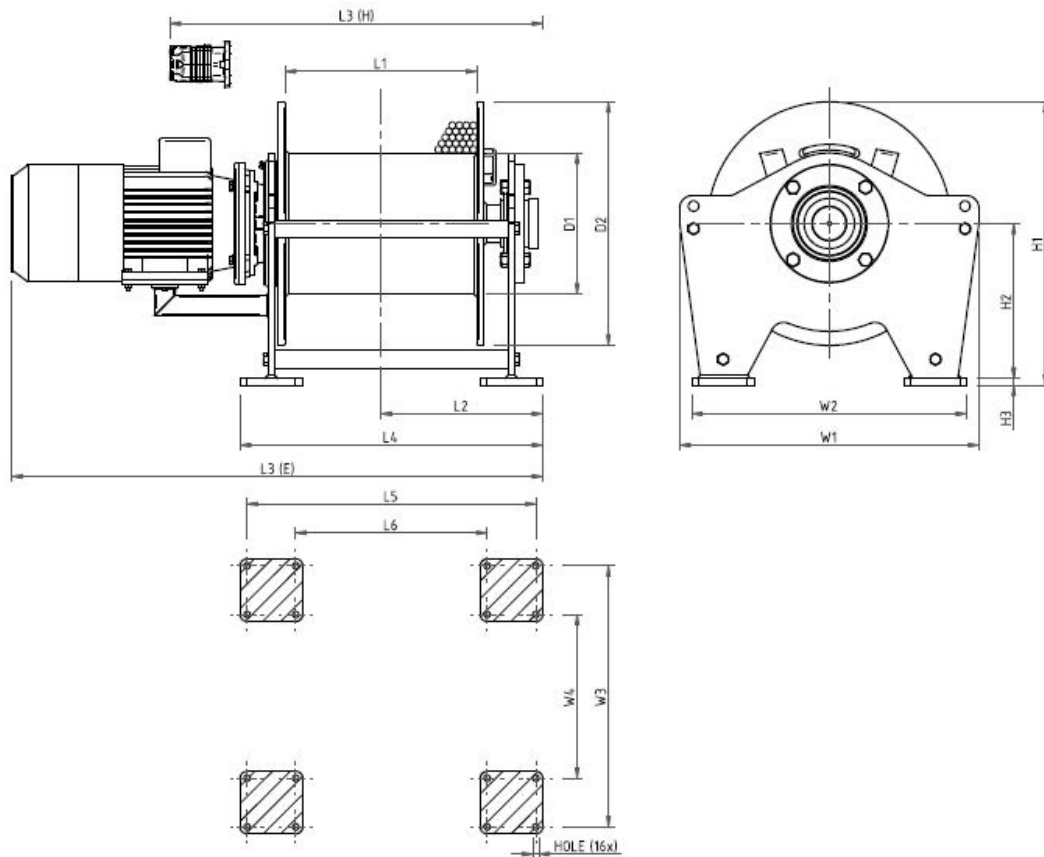
FOOTPRINT -TOP VIEW- A-A
