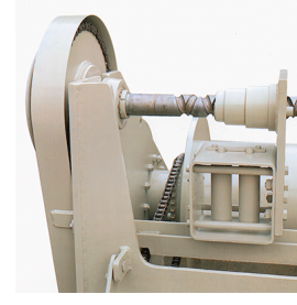
SPOOLING GEAR
